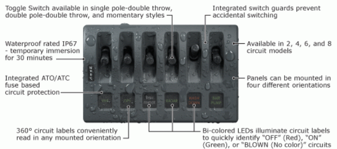
BLUE SEA WATER PROOF FUSE PANELS 12V E824304 4 POSITION E824306 6 POSITION E824308 8 POSITION
