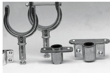
ROWLOCKS TOP SOCKET SIDE SOCKET ALLOY 17mm x 56mm T/SOCKET N29610 48mm 10.88 N29614 8.39 N29612 5.15 N13372 9.90 N13373 8.03 N29611 58mm 13.36 N29615 8.24 N29613 9.98 SIDE SOCKET N13374
