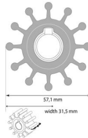
F5 NEOPRENE 57.1mm x 31.5mm wide JOHNSON A09-801B 31.67 JABSCO A4568-0001 48.00 NITRILE LARGE DIA CENT JOHNSON A 09-804B-9 75.67
