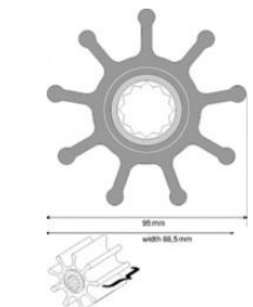
F9 NEOPRENE IMPELLER 95mm x 88.5mm w 9 VANES JOHNSON A09-802b 112.27 JABSCO A6760-0001 9 VANES
