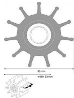
F8 95mm x 63mm wide NEOPRENE JOHNSON A09-819B 64.50 JABSCO A836-0001 40.51 NITRILE A09-819-B-9 65.65 A836-0003 40.51 09-819B & B-9 SUPERCEDES 09-1029B
