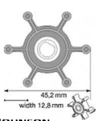
JOHNSON F3 NITRILE IMPELLER A09-1052-9 24.00 45.2mm x 12.8 wide
