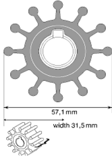
F5 NEOPRENE 57.1mm x 31.5mm wide JOHNSON A09-801B 34.85 JABSCO A4568-0001 48.00 NITRILE LARGE DIA CENT JOHNSON A09-804B-9 75.67
