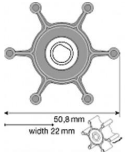
F4 50.8 22mm wide D shaft NITRILE JOHNSON A09-824P-9 23.16 JABSCO A6303-0003 24.96
