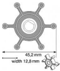
JOHNSON F3 NITRILE IMPELLER A09-1052-9 25.33 45.2mm x 12.8 wide
