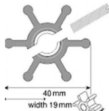
JOHNSON (MC97) F35 IMPELLER 40mm x 19mm A09-806B 20.27 A4528-000 JABSCO 22.33
