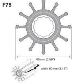
F75 65mm x 80mm wide NEOPRENE JOHNSON A09-812B-1 39.74 JABSCO A13554-0001 40.56
