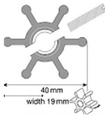
JOHNSON (MC97) F35 IMPELLER 40mm x 19mm A09-806B 22.62 A4528-000 JABSCO 22.33
