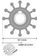
F5 NEOPRENE 57.1mm x 31.5mm wide JOHNSON A09-801B 31.67 JABSCO A4568-0001 48.00 NITRILE LARGE DIA CENT JOHNSON A 09-804B-9 75.67
