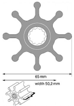
F7 65mm x 50.2 mm wide Neoprene JOHNSON A09-1028B 44.34 JABSCO A17937-0001 32.33 NITRILE JOHNSON A09-1028B-9 43.18 JABSCO A17937-0003 32.33
