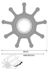
F9 NEOPRENE IMPELLER 95mm x 88.5mm w 9 VANES JOHNSON A09-802b 112.27 JABSCO A6760-0001 9 VANES
