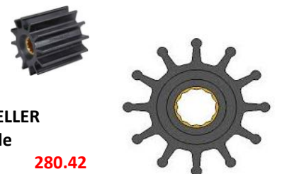
F8 95mm x 63mm wide NEOPRENE JOHNSON A09-819B 64.50 JABSCO A836-0001 40.51 NITRILE A09-819-B-9 65.65 A836-0003 40.51 09-819B & B-9 SUPERCEDES 09-1029B
