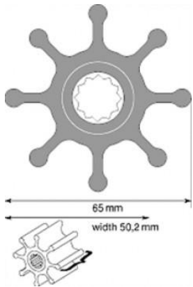
F7 65mm x 50.2 mm wide Neoprene JOHNSON A09-1028B 44.34 JABSCO A17937-0001 32.33 NITRILE JOHNSON A09-1028B-9 43.18 JABSCO A17937-0003 32.33
