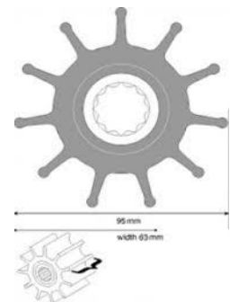
F8 95mm x 63mm wide NEOPRENE JOHNSON A09-819B 64.50 JABSCO A836-0001 40.51 NITRILE A09-819-B-9 65.65 A836-0003 40.51 09-819B & B-9 SUPERCEDES 09-1029B
