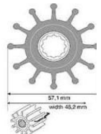
F 6 MC97 57mm x 48.2mm JOHNSON A09-812B-1 39.74 JABSCO A13554-0001 48.67
