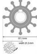
F5 NEOPRENE 57.1mm x 31.5mm wide JOHNSON A09-801B 34.85 JABSCO A4568-0001 48.00 NITRILE LARGE DIA CENT JOHNSON A09-804B-9 75.67
