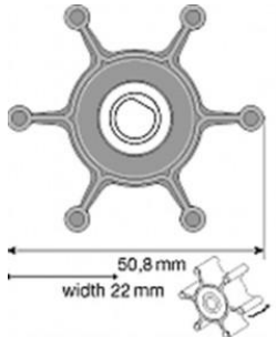
F4 50.8 22mm wide D shaft NITRILE JOHNSON A09-824P-9 24.72 JABSCO A6303-0003 24.37
