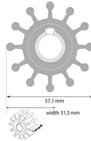
F5 NEOPRENE 57.1mm x 31.5mm wide JOHNSON A09-801B 34.85 JABSCO A4568-0001 48.00 NITRILE LARGE DIA CENT JOHNSON A09-804B-9 75.67
