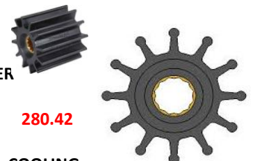
F8 95mm x 63mm wide NEOPRENE JOHNSON A09-819B 64.50 JABSCO A836-0001 40.51 NITRILE A09-819-B-9 65.65 A836-0003 40.51 09-819B & B-9 SUPERCEDES 09-1029B
