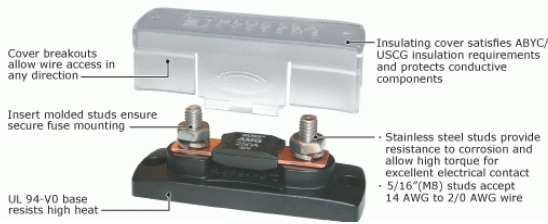
ANL FUSE BLOCK 35 -300 AMP WITH COVER E825005 31.79 BLUESEA
