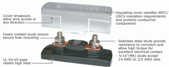
ANL FUSE BLOCK 35 - 300 AMP WITH COVER E825005 32.08 BLUESEA
