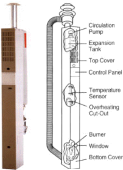
ALDE COMPACT BOILER F29100
