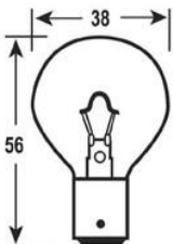
GOLF BALL BS15D SBC DC L813088 12V 24 W 2.47
