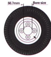
TRAILER WHEEL & TYRE 4 STUD ON 4" T470 400 X 8 38.72 T471 500 X 10 57.60
