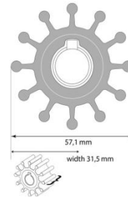
F5 MC97 57.1mm X 31.5mm wide JOHNSON 09-1027B 28.57 JABSCO 1210-0001 NITRILE JOHNSON 09-1027B-9 30.56 JABSCO 1210-003
