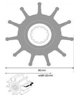
F6 95mm x 63mm wide NEOPRENE JOHNSON 09-819B 60.86 JABSCO 836-0001 40.51 NITRILE JOHNSON 09-819-B-9 61.99 JABSCO 836-0003 40.51 09-819B & B-9 SUPERCEDES 09-1029B
