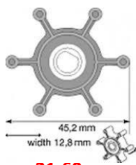
21.60 F3 NITRILE IMPELLER JOHNSON 09-1052-9 45.2mm x 12.8 wide
