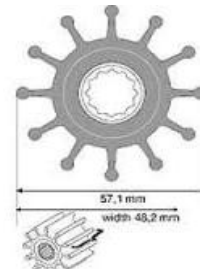
F6 MC97 57mm x 48.2mm JOHNSON 09-812B-1 37.62 JABSCO 13554-0001
