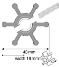
17.58 F35 IMPELLER 40mm x 19mm JOHNSON (MC97) 09-806B JABSCO 4528-0001 21.80
