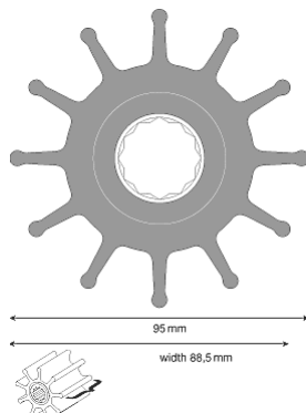
F9 NEOPRENE IMPELLER 95mm x 88.5mm 12 vanes JOHNSON 09-814 106.45 JABSCO 21676-0001
