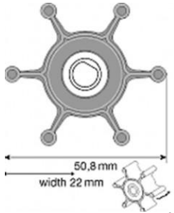
F4 50.8 22mm wide D shaft NITRILE JOHNSON 09-824P-9 21.24 JABSCO 6303-0003 24.37
