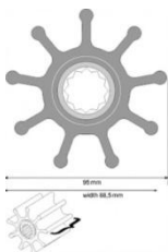
F9 NEOPRENE IMPELLER 95mm x 88.5mm w 9 VANES JOHNSON 09-802b 106.25 JABSCO 6760-0001 9 VANES
