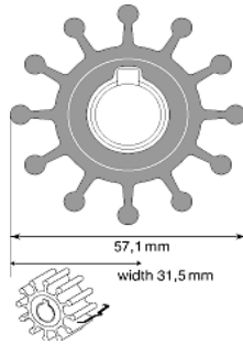
F5 NEOPRENE 57.1mm x 31.5mm wide JOHNSON 09-801B 29.76 JABSCO 4568-0001 34.09 NITRILE LARGE DIA CENT JOHNSON 09-804B-9 66.41
