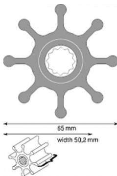
F7 65mm x 50.2 mm wide Neoprene JOHNSON 09-1028B 40.93 JABSCO 17937-0001 31.57 NITRILE JOHNSON 09-1028B-9 40.93 JABSCO 17937-0003 31.57
